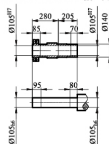
KH/ KHZ/ KHF127输出轴
