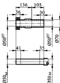
KH/ KHZ/ KHF77输出轴
