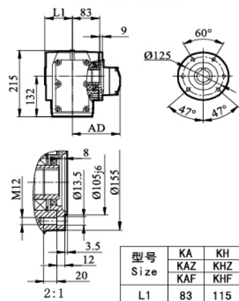
KAF / KHF / KV57
