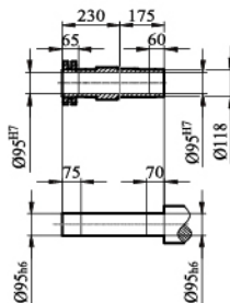
KH/ KHZ/ KHF107输出轴
