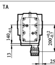
KH/ KHZ/ KHF67输出轴
