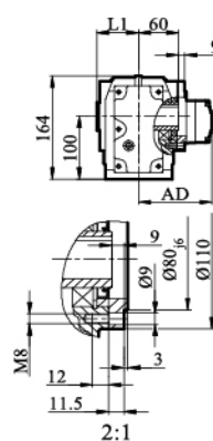
KAF/ KHF/ KVH37
