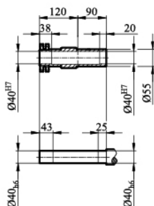
KH/ KHZ/ KHF67输出轴
