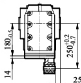
KH/ KHZ/ KHF77输出轴
