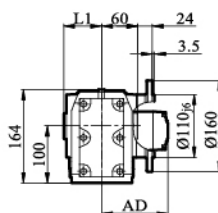
KAF/ KHF/ KVH37
