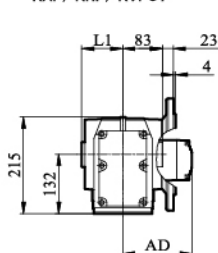
KAF / KHF / KV57
